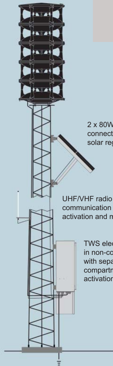
TWS295 SIREN WITH SOLAR POWER AND RADIO LINK
